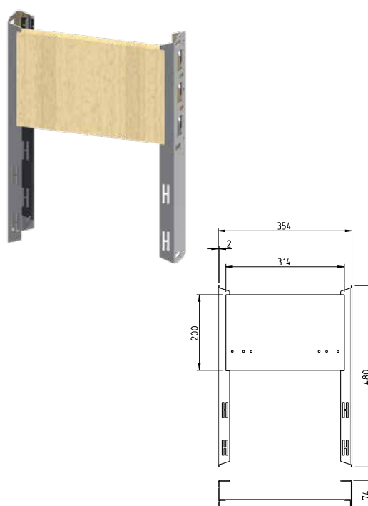
Figur WT222 - Traverse
