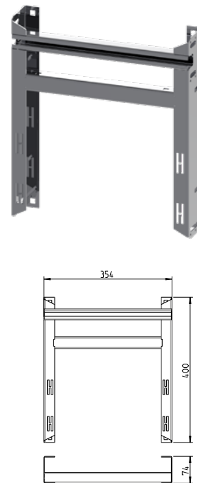
Figur WT212 - Traverse
